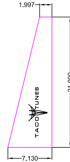
Right Side Panel Face Elevation View
