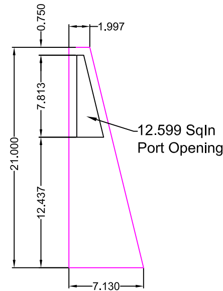
Left Side Panel Face Elevation View
