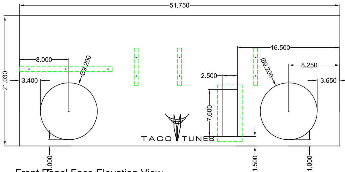
Front Panel Face Elevation View
