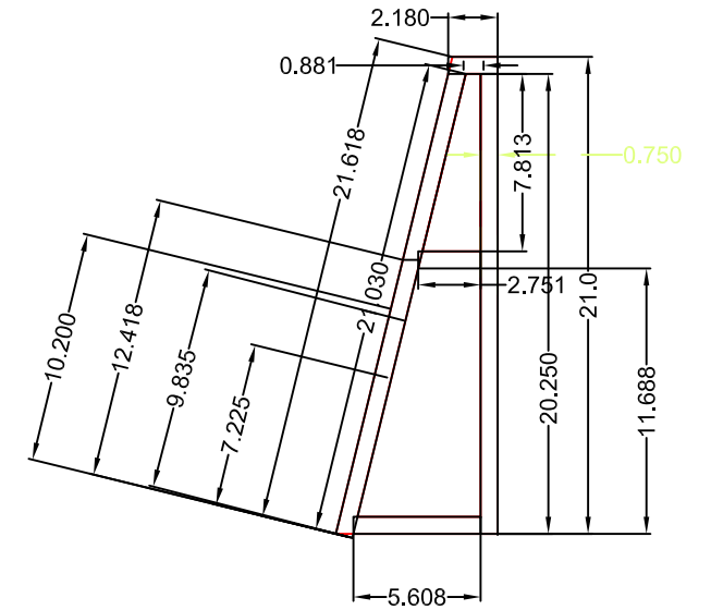
1- Section View Assembly (untrimmed)
