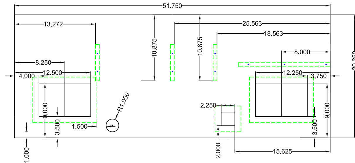
Back Panel Face Elevation View (View from backside of box)
