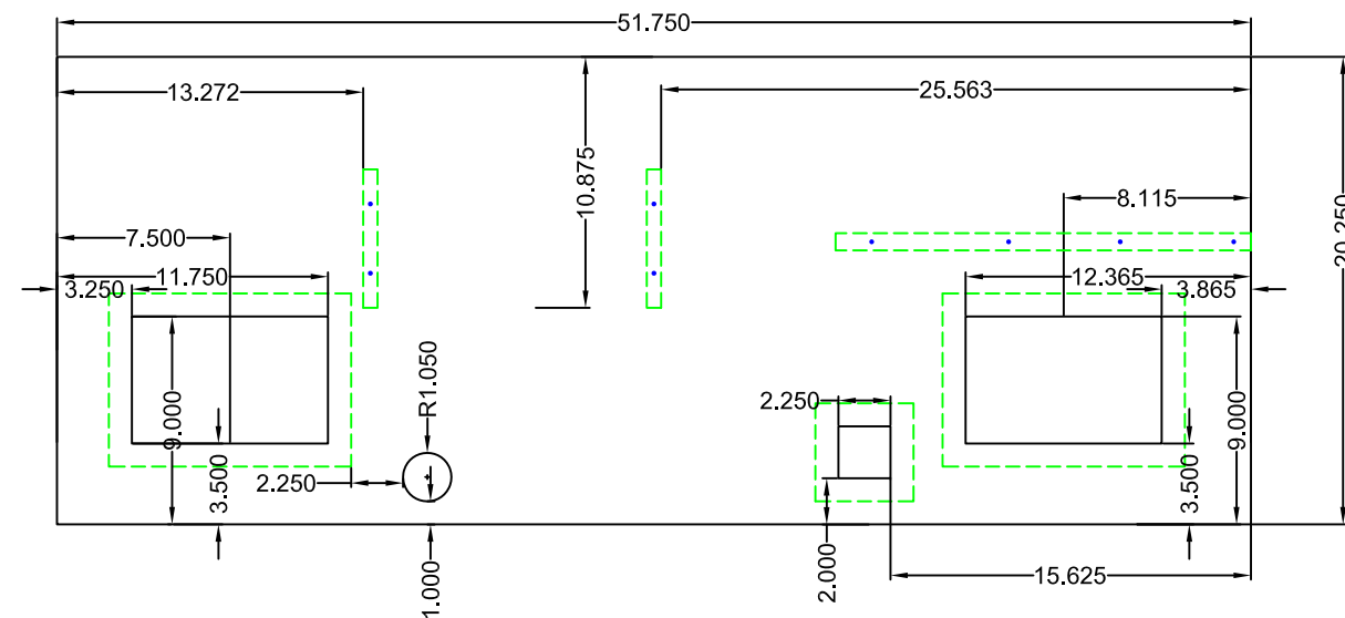
Back Panel Face Elevation View (View from backside of box)
