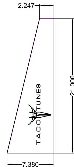
Right Side Panel Face Elevation View
