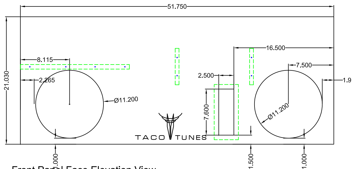
Front Panel Face Elevation View
