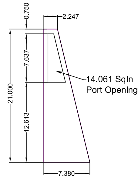
Left Side Panel Face Elevation View
