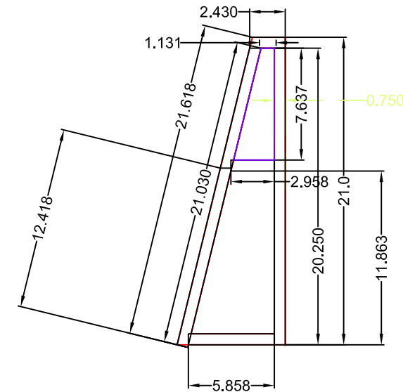
1- Section View Assembly (untrimmed)
