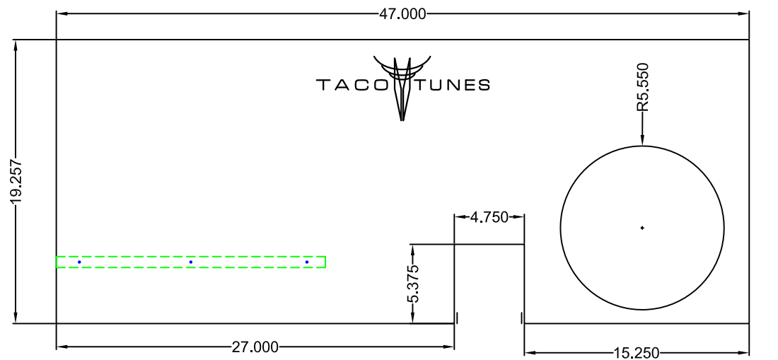
Front Panel Face Elevation View
