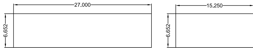
Bottom Panels Face Elevation View
