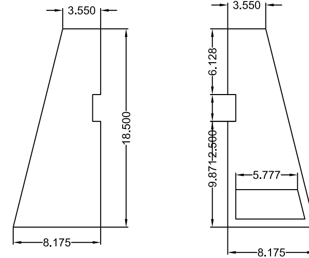
Right and Left Side Panels Face Elevation View
