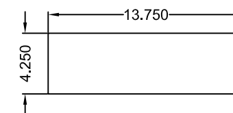
Interior Cover Pieces (2 pcs) 1/4" MDF Thickness
