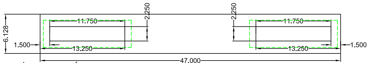
Bottom Panels Face Elevation View
