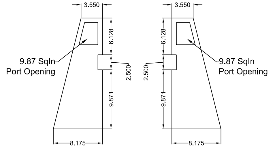
Right and Left Side Panels Face Elevation View
