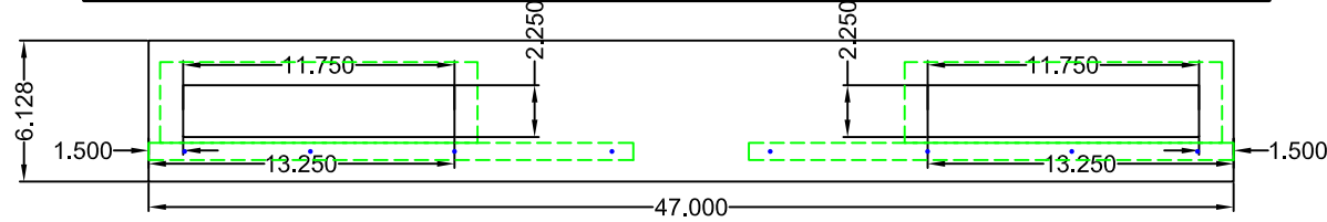
Bottom Panels Face Elevation View
