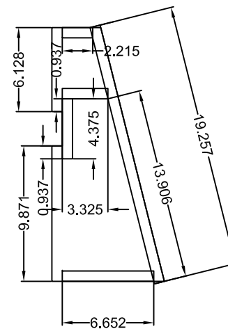
1- Section View Assembly (untrimmed)
