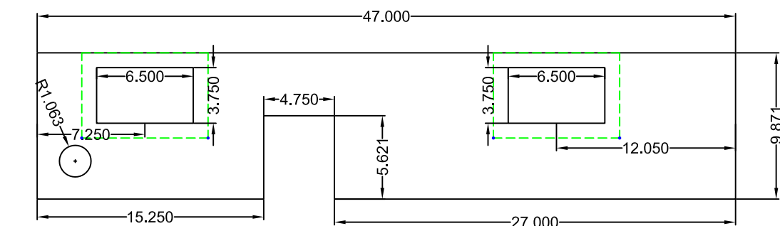
Back Panels Face Elevation View (View from backside of box)
