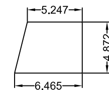
Bottom Upright Pieces (2 pcs)
