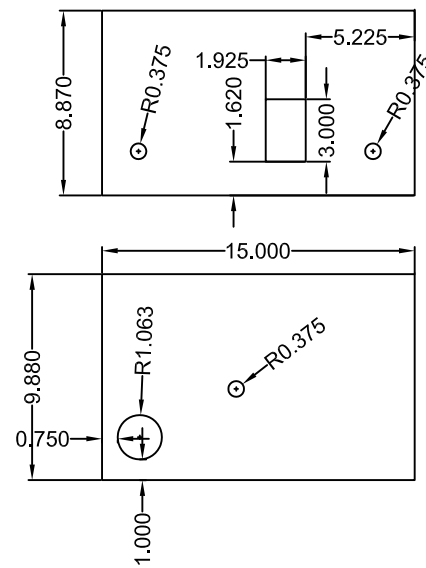
Back Panels Face Elevation View (View from backside of box)
