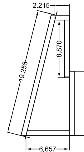
Right and Left Side Panels Face Elevation View
