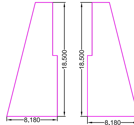
Right and Left Side Panels Face Elevation View
